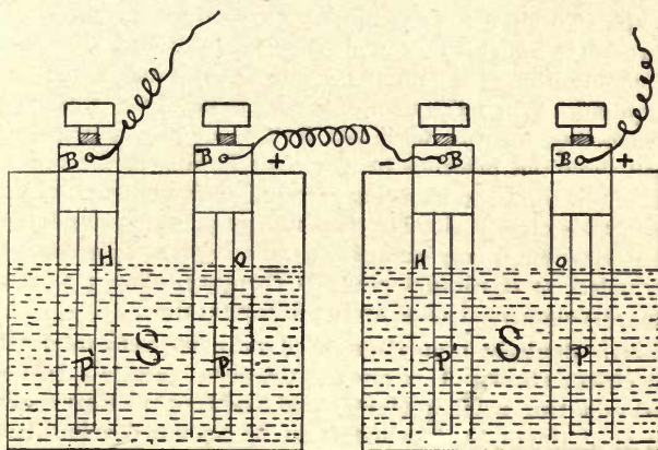
Fig. 44. GAS BATTERY.
